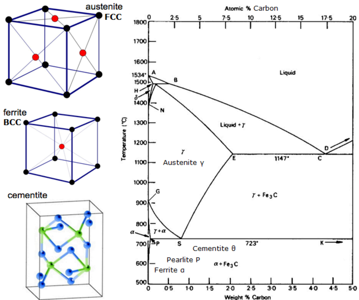
Lattice structures on steel showing the relationship of the various phases of state as a function of impurity composition / percentage for alloyed iron.
